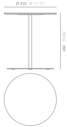
MIOM laquered MDF top and "O" base
