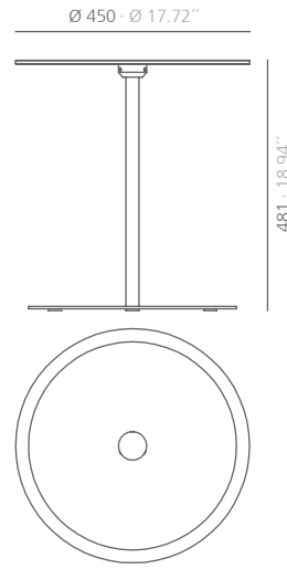
MIOC 10mm glass top and base "O" base
