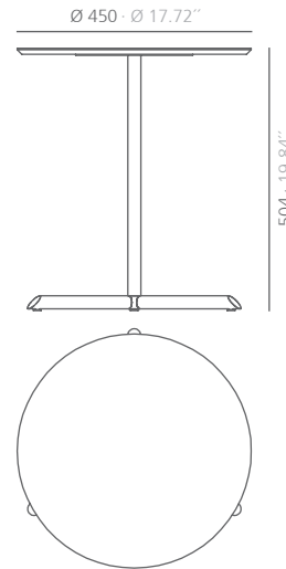
MIYM laquered MDF top and "Y" base
