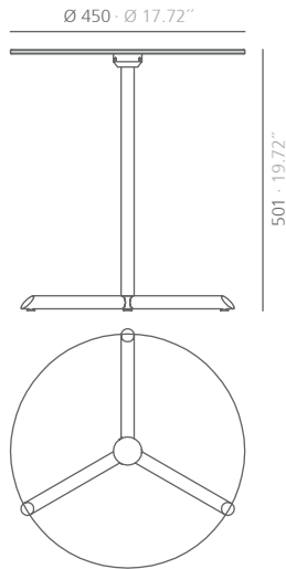
MIYC 10mm glass top and "Y" base
