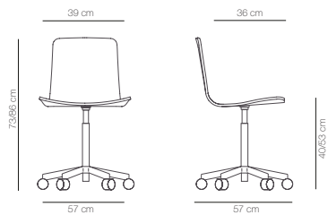
Casters base
