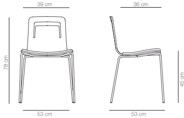
4 legs
