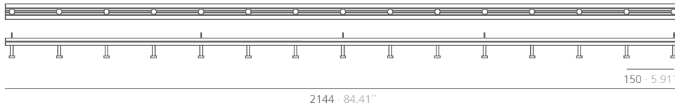
CLI15 15 hangers
